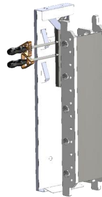
Charger Assy, 12-Probe Linear Side Oven Mtg
